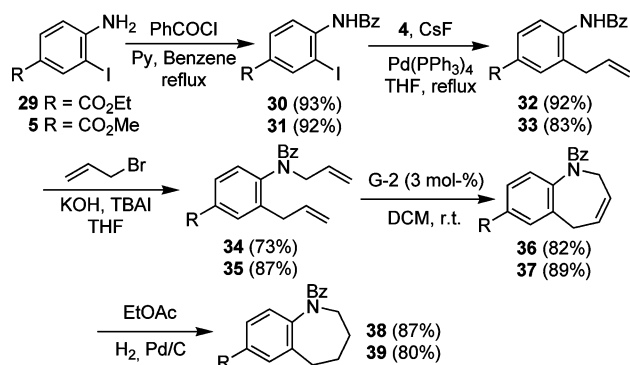
Scheme 3. Synthetic approach to 1-benzazepine derivatives with N -benzoyl protection.
