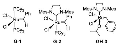
Figure 2. Ruthenium carbene metathesis catalysts.
