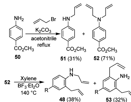
Scheme 6. Synthesis of diallyl derivative 48 by the aza-Claisen rearrangement.
