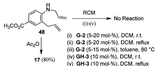
Scheme 7. Attempted RCM conditions and N -acetyl protection of the diallyl derivative 48 .
