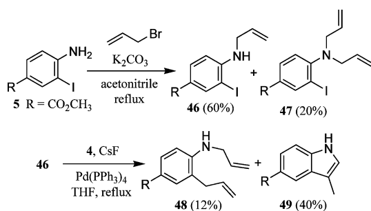
Scheme 5. Synthesis of 7-substituted 1H-1-benzazepine derivatives by SM cross-coupling.
