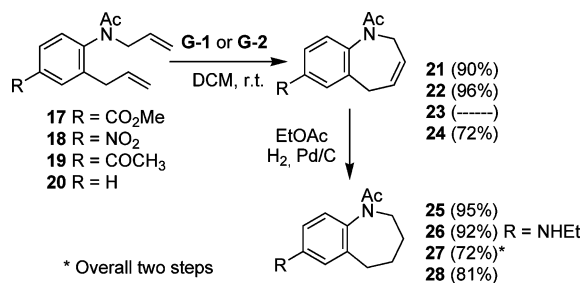
Scheme 2. Synthesis of 1-benzazepine derivatives by RCM and hydrogenation.
