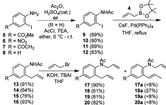
Scheme 1. Preparation of diallyl derivatives by the SM cross-coupling reaction as a key step.
