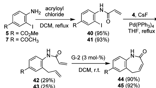
Scheme 4. Synthesis of 1-benzazepine-2-one derivatives without N -protection.
